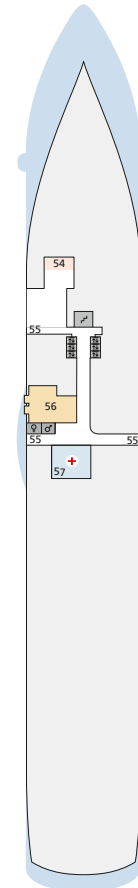
Deck 3 54 Bikingstation, Tauchbasis 55 Gangway/ Tenderporten 56 Pier 3 Bar 57 Hospital
